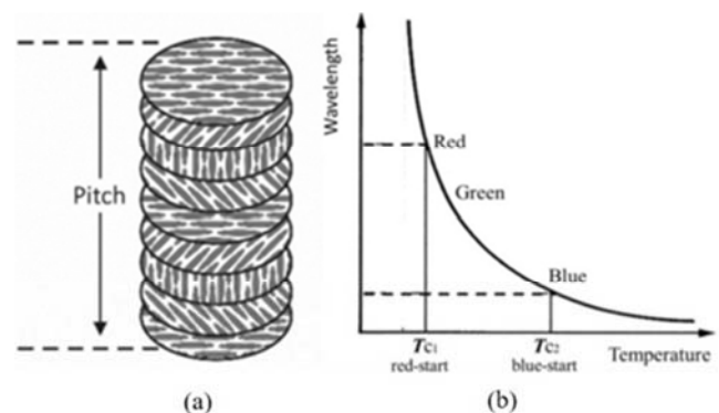
Figure 1. (a) Molecules alignment of chiral nematic liquid crystal structure. (b) The Graph of reflected wavelengths against the temperatures [3].
